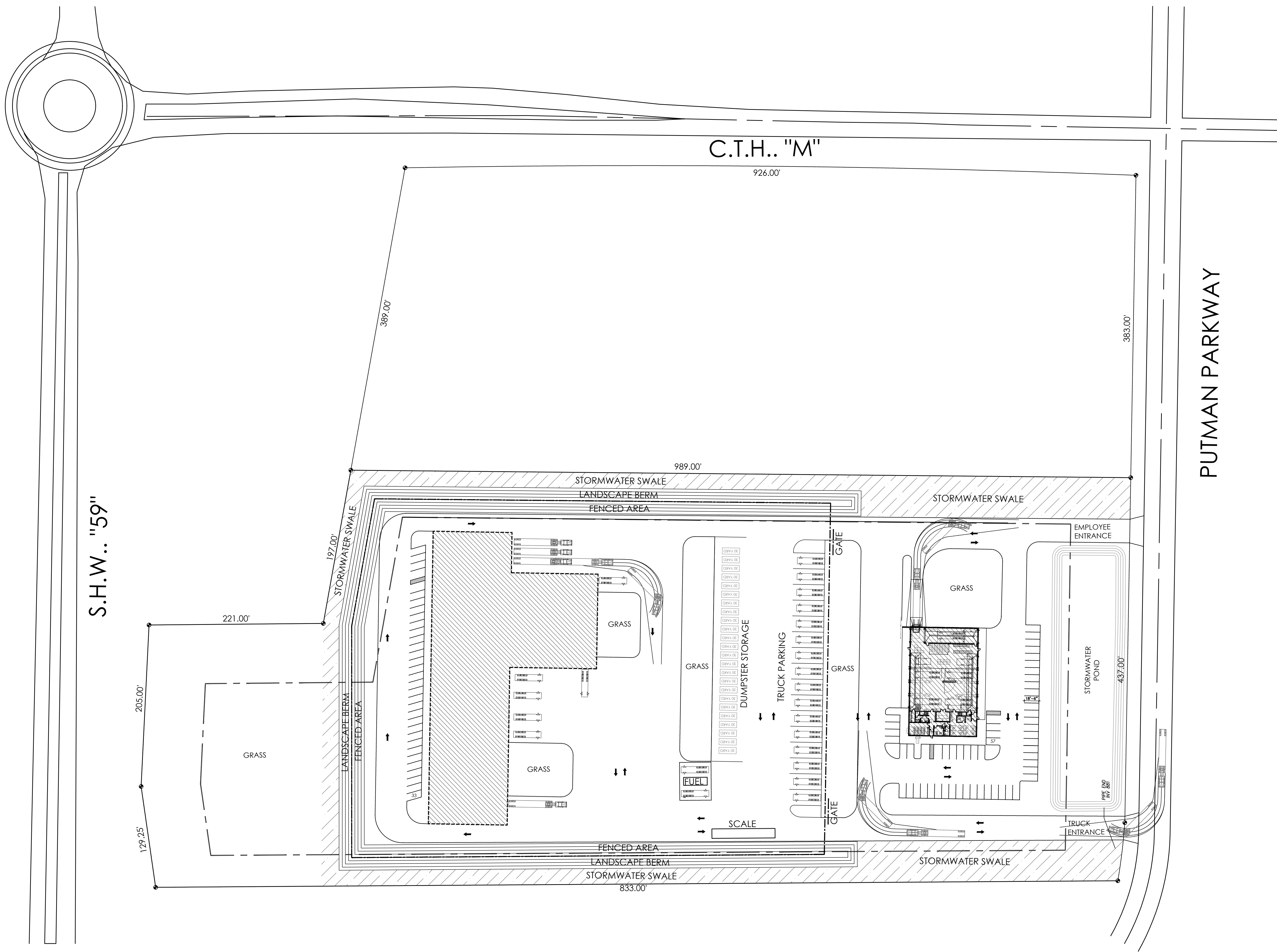
⊖ ARCH. SITE PLAN 1" = 60'-0"
