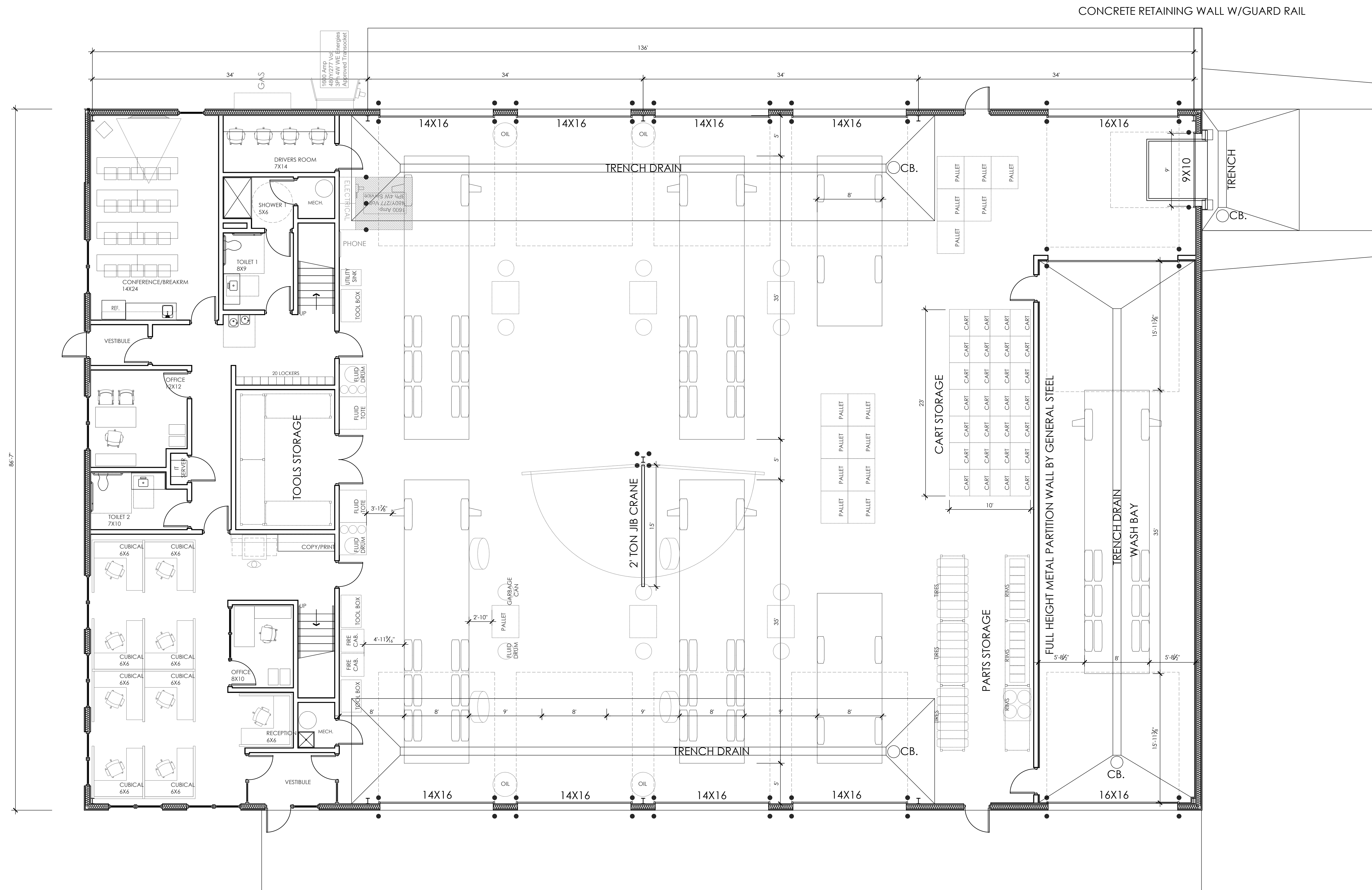
FIRST FLOOR PLAN 1/8" = 1'-0" FIRST FLOOR - 11,995 sqft.
